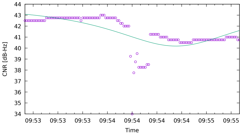
CNR fit for G22 on Xiaomi11T - drive 9 (DOY263)
