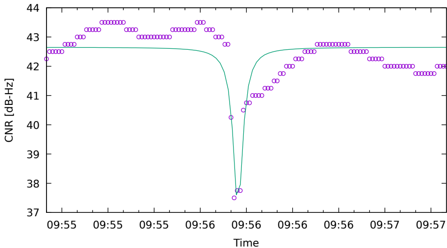
CNR fit for G31 on Xiaomi11T - drive 10 (DOY263)
