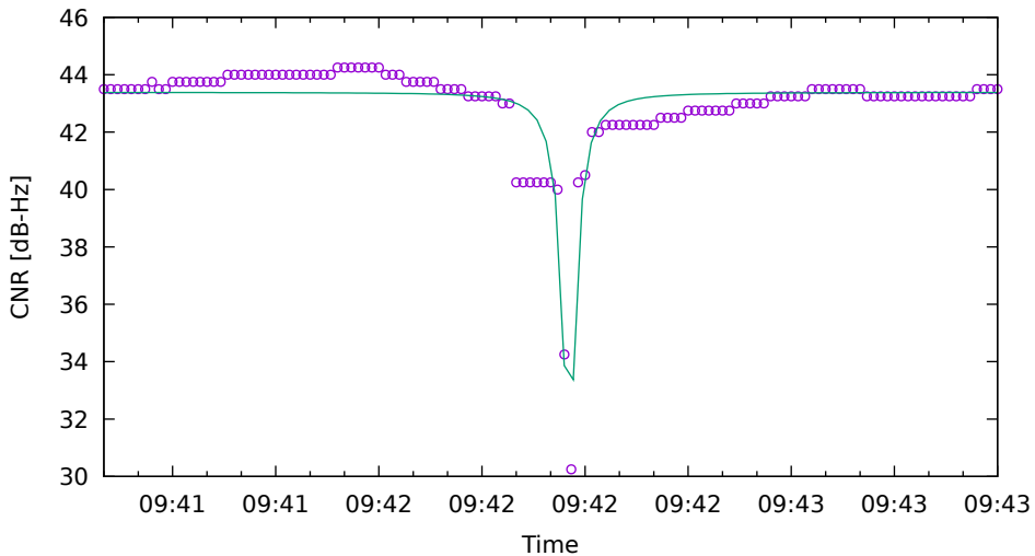
CNR fit for G31 on Xiaomi11T - drive 2 (DOY263)
