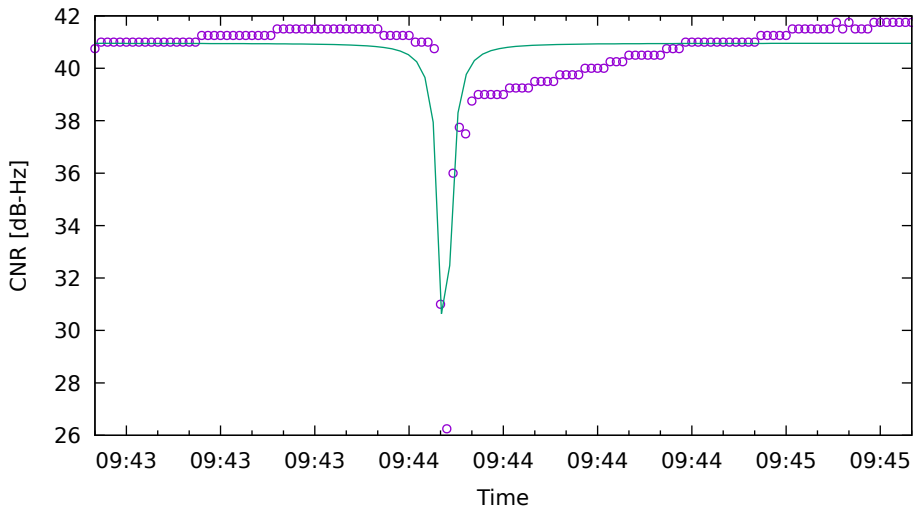
CNR fit for G32 on Xiaomi11T - drive 3 (DOY263)
