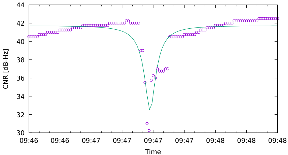
CNR fit for G32 on Xiaomi11T - drive 5 (DOY263)
