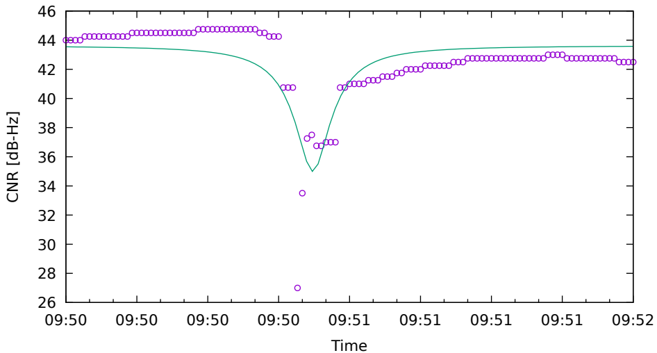
CNR fit for G32 on Xiaomi11T - drive 7 (DOY263)
