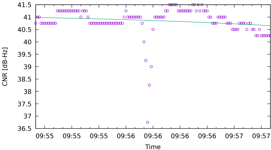
CNR fit for C11 on XiaomiMi8 - drive 10 (DOY263)
