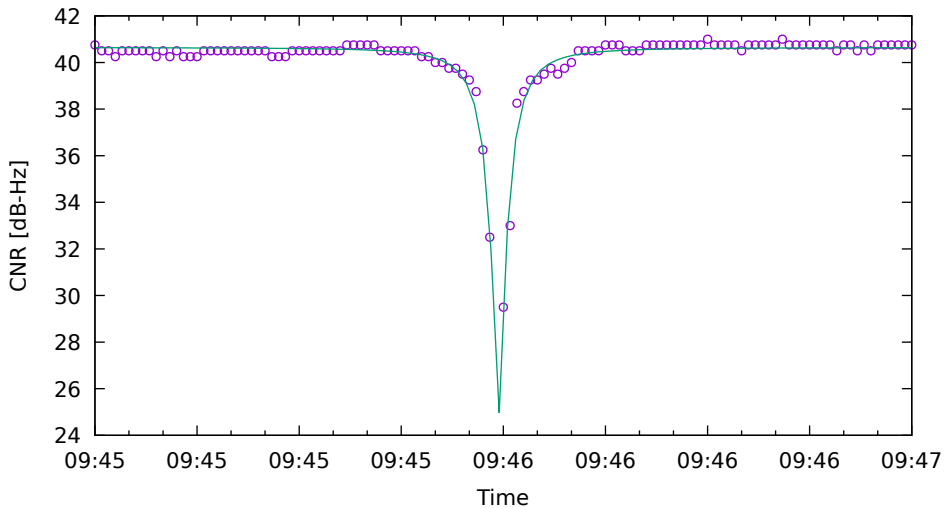
CNR fit for C11 on XiaomiMi8 - drive 4 (DOY263)
