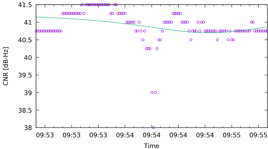
CNR fit for C11 on XiaomiMi8 - drive 9 (DOY263)
