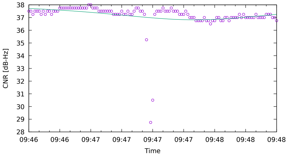
CNR fit for C12 on XiaomiMi8 - drive 5 (DOY263)
