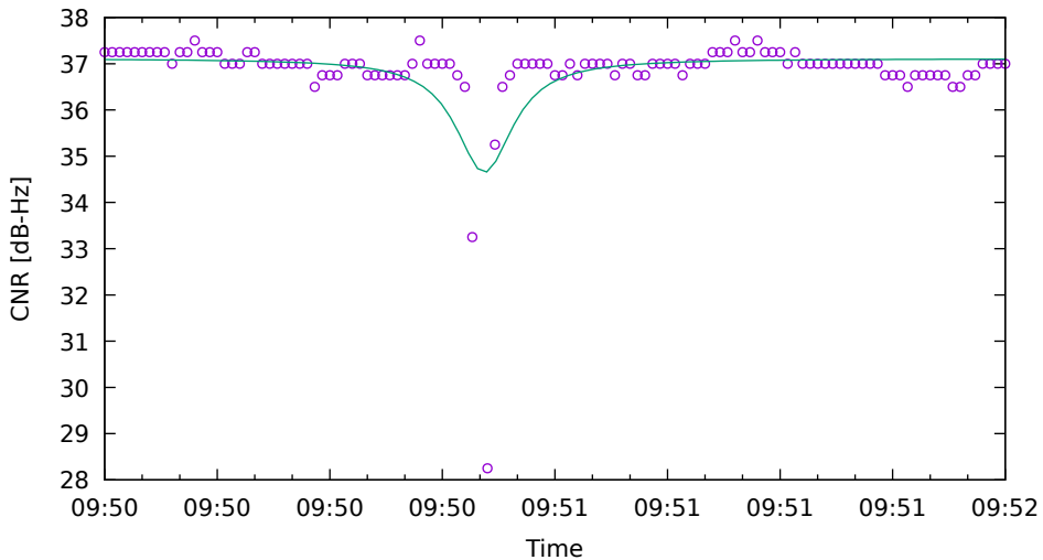
CNR fit for C12 on XiaomiMi8 - drive 7 (DOY263)
