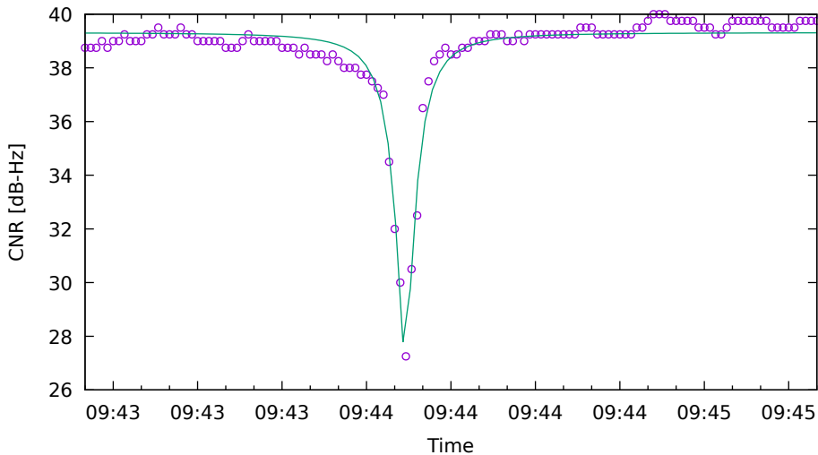
CNR fit for C21 on XiaomiMi8 - drive 3 (DOY263)
