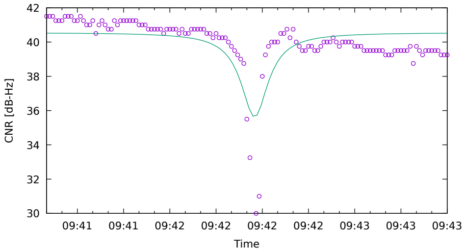
CNR fit for C28 on XiaomiMi8 - drive 2 (DOY263)
