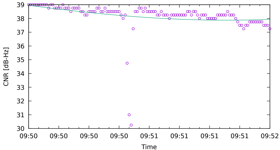
CNR fit for C34 on XiaomiMi8 - drive 7 (DOY263)
