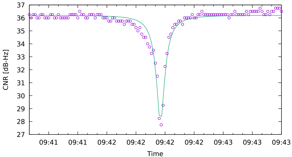
CNR fit for E04 on XiaomiMi8 - drive 2 (DOY263)
