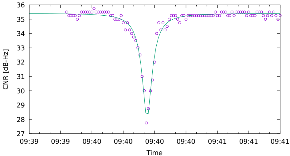
CNR fit for E19 on XiaomiMi8 - drive 1 (DOY263)
