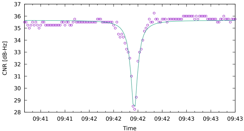
CNR fit for E19 on XiaomiMi8 - drive 2 (DOY263)
