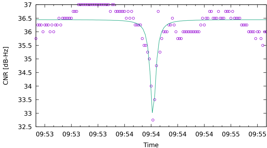
CNR fit for E33 on XiaomiMi8 - drive 9 (DOY263)
