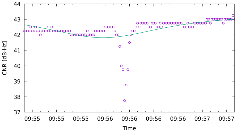
CNR fit for G03 on XiaomiMi8 - drive 10 (DOY263)
