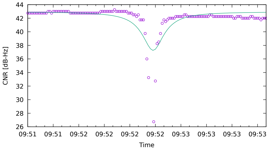
CNR fit for G03 on XiaomiMi8 - drive 8 (DOY263)
