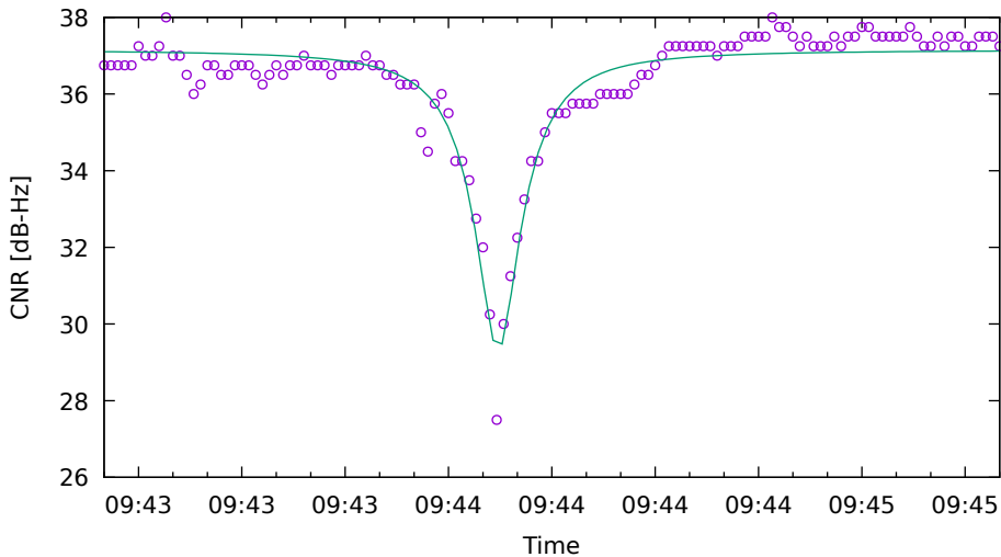
CNR fit for G04 on XiaomiMi8 - drive 3 (DOY263)
