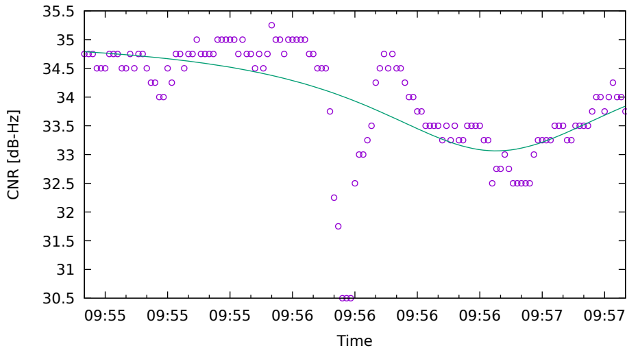
CNR fit for G08 on XiaomiMi8 - drive 10 (DOY263)
