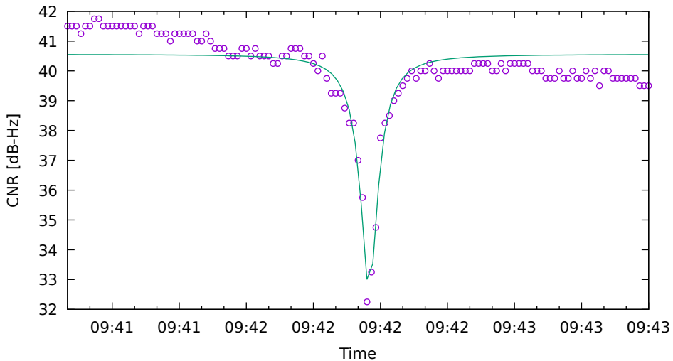
CNR fit for G08 on XiaomiMi8 - drive 2 (DOY263)
