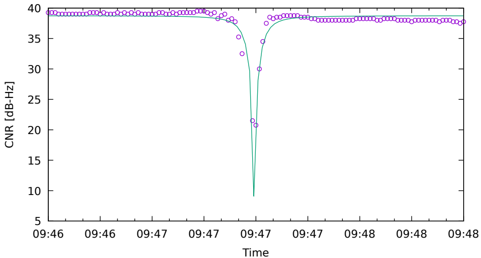
CNR fit for G08 on XiaomiMi8 - drive 5 (DOY263)
