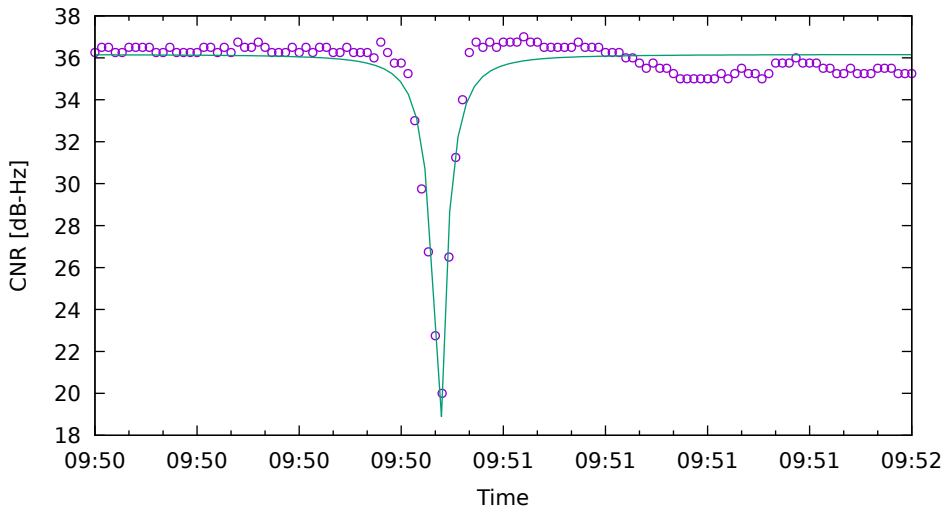
CNR fit for G08 on XiaomiMi8 - drive 7 (DOY263)
