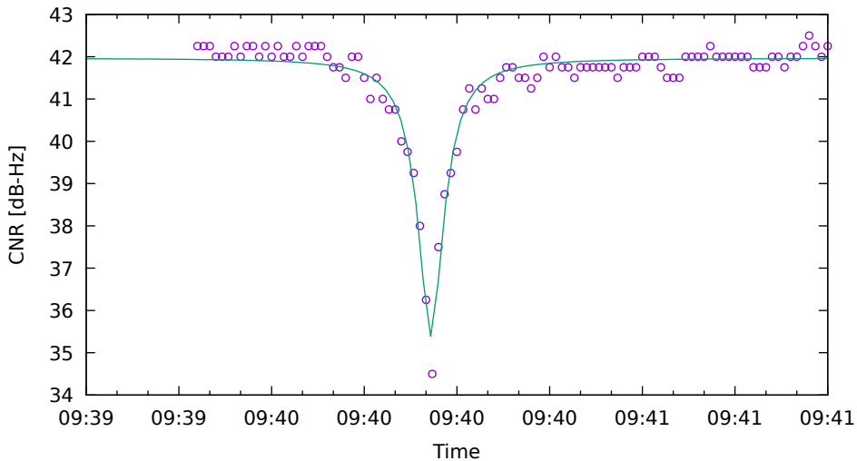
CNR fit for G17 on XiaomiMi8 - drive 1 (DOY263)
