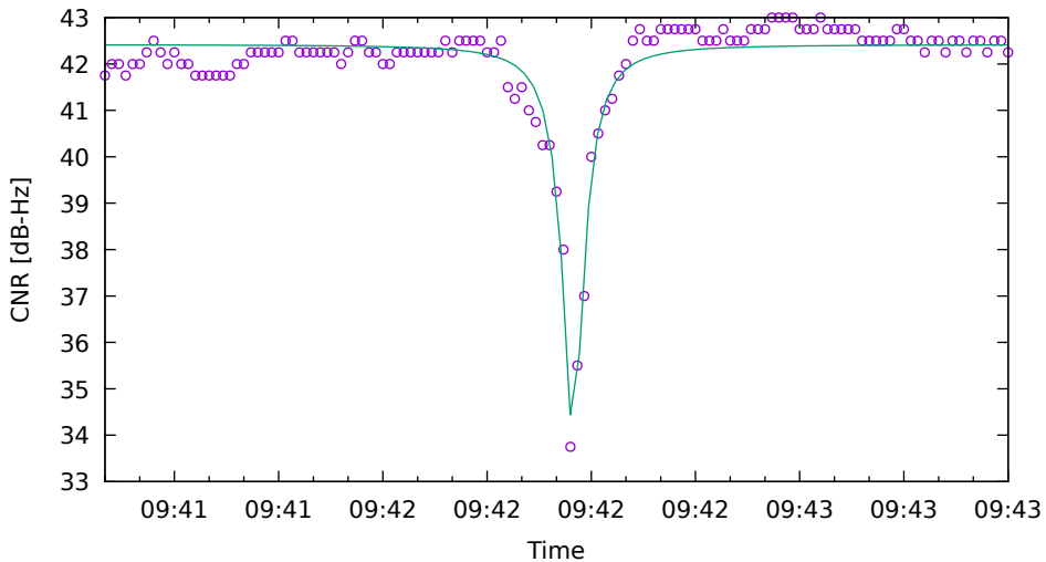
CNR fit for G17 on XiaomiMi8 - drive 2 (DOY263)
