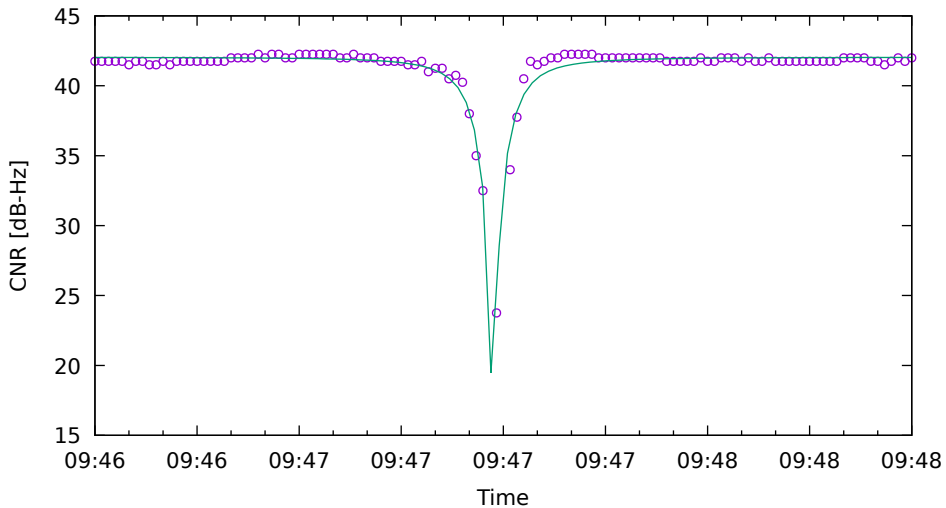
CNR fit for G17 on XiaomiMi8 - drive 5 (DOY263)
