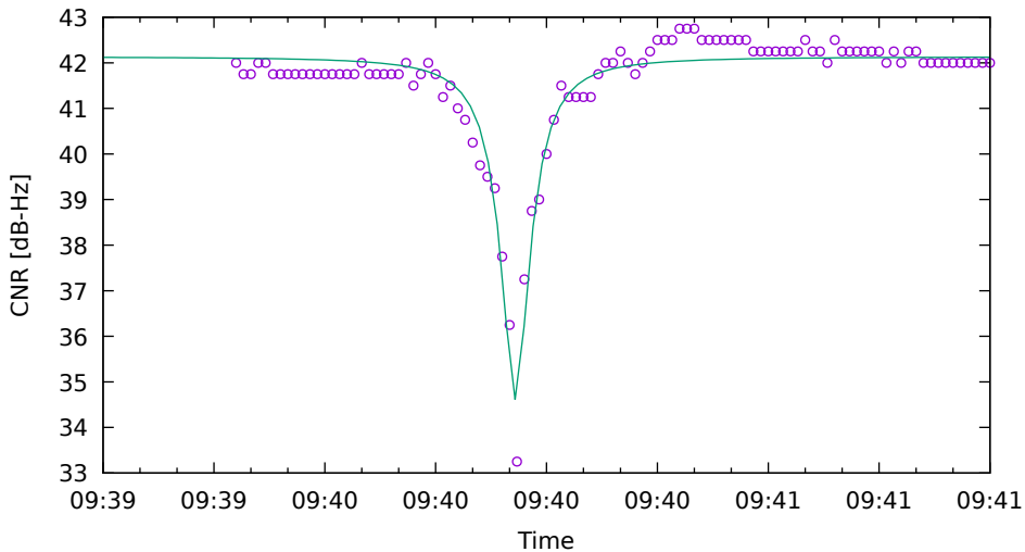
CNR fit for G19 on XiaomiMi8 - drive 1 (DOY263)
