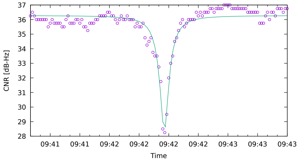
CNR fit for G22 on XiaomiMi8 - drive 2 (DOY263)
