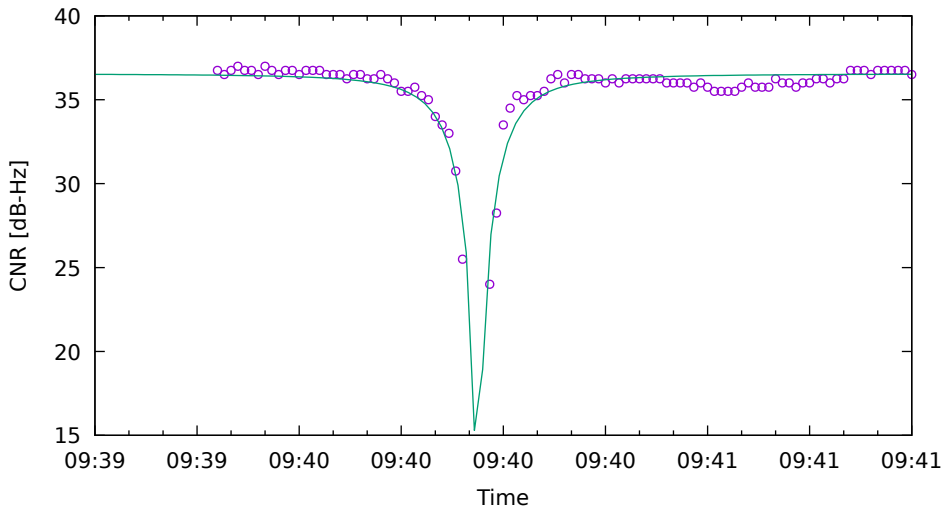
CNR fit for R01 on XiaomiMi8 - drive 1 (DOY263)
