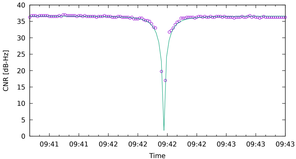
CNR fit for R01 on XiaomiMi8 - drive 2 (DOY263)
