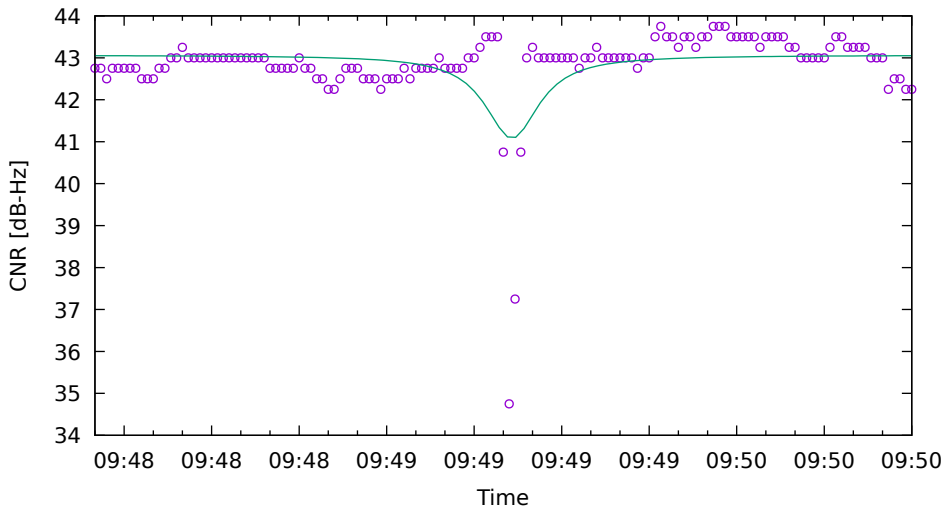
CNR fit for R02 on XiaomiMi8 - drive 6 (DOY263)
