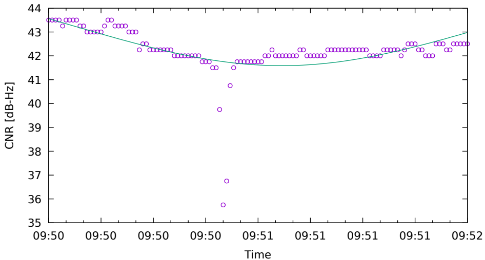
CNR fit for R02 on XiaomiMi8 - drive 7 (DOY263)
