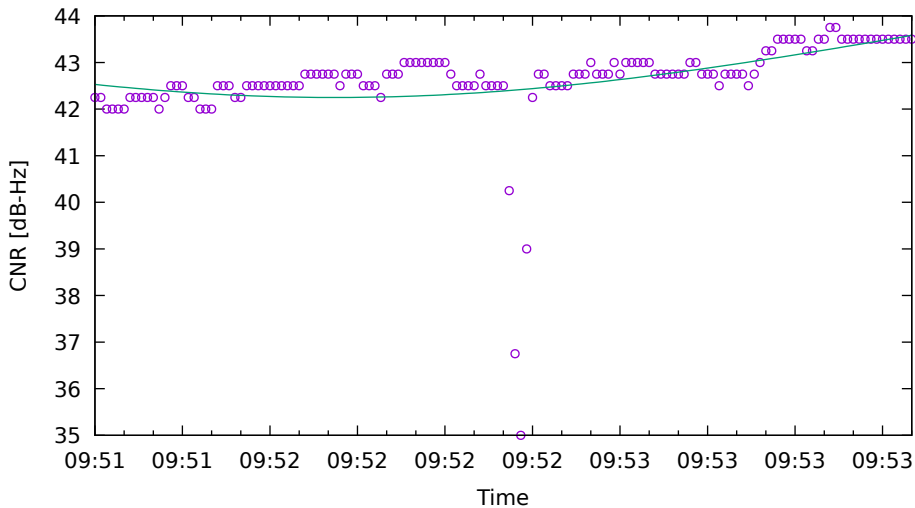
CNR fit for R02 on XiaomiMi8 - drive 8 (DOY263)
