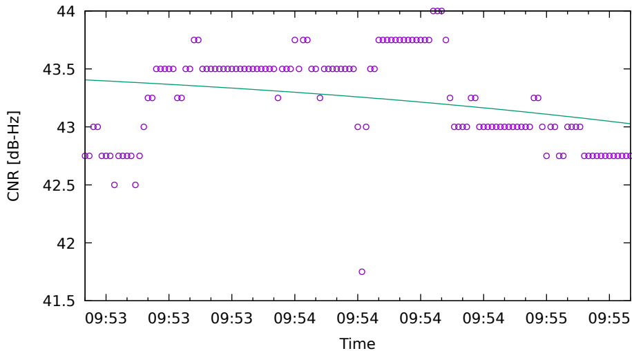
CNR fit for R02 on XiaomiMi8 - drive 9 (DOY263)
