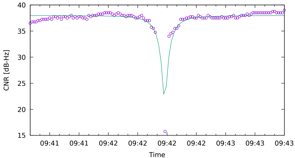
CNR fit for R23 on XiaomiMi8 - drive 2 (DOY263)
