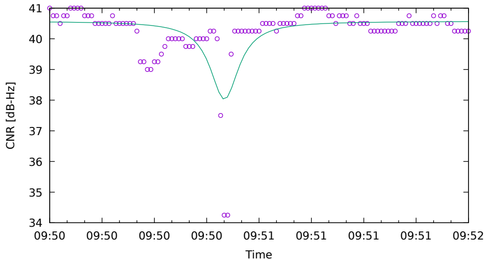
CNR fit for R24 on XiaomiMi8 - drive 7 (DOY263)
