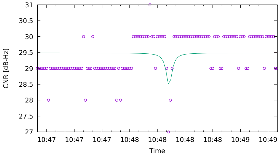
CNR fit for C09 on HuaweiP40 - drive 5 (DOY263)
