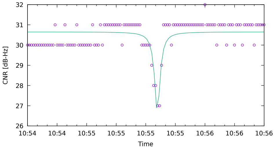
CNR fit for C09 on HuaweiP40 - drive 9 (DOY263)
