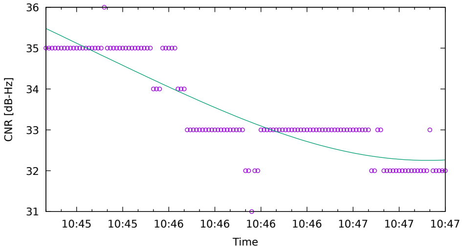
CNR fit for C14 on HuaweiP40 - drive 4 (DOY263)
