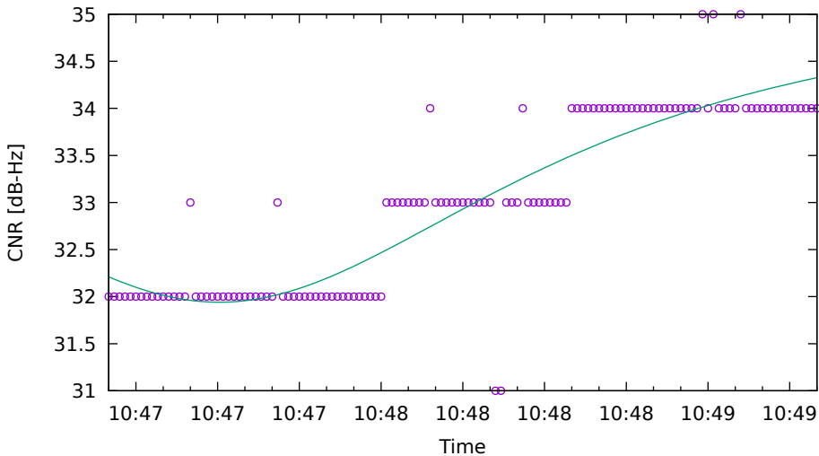
CNR fit for C14 on HuaweiP40 - drive 5 (DOY263)
