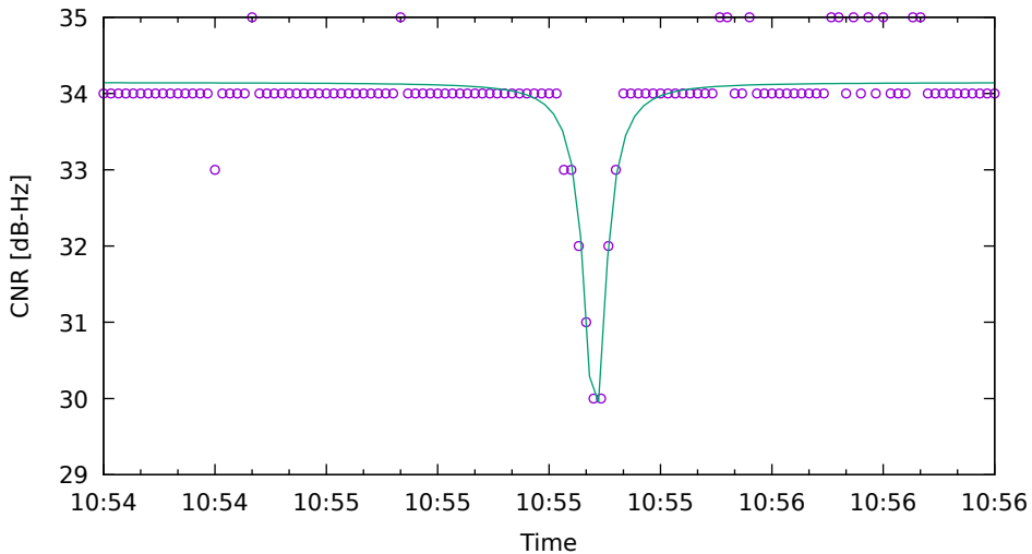
CNR fit for C14 on HuaweiP40 - drive 9 (DOY263)
