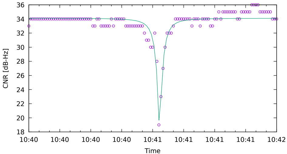
CNR fit for G01 on HuaweiP40 - drive 1 (DOY263)
