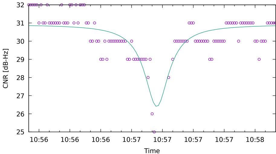
CNR fit for G01 on HuaweiP40 - drive 10 (DOY263)
