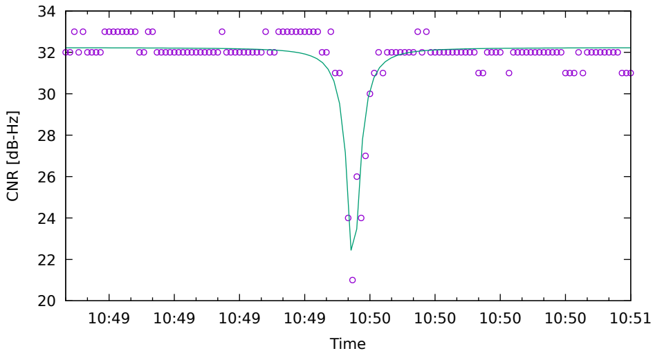
CNR fit for G01 on HuaweiP40 - drive 6 (DOY263)
