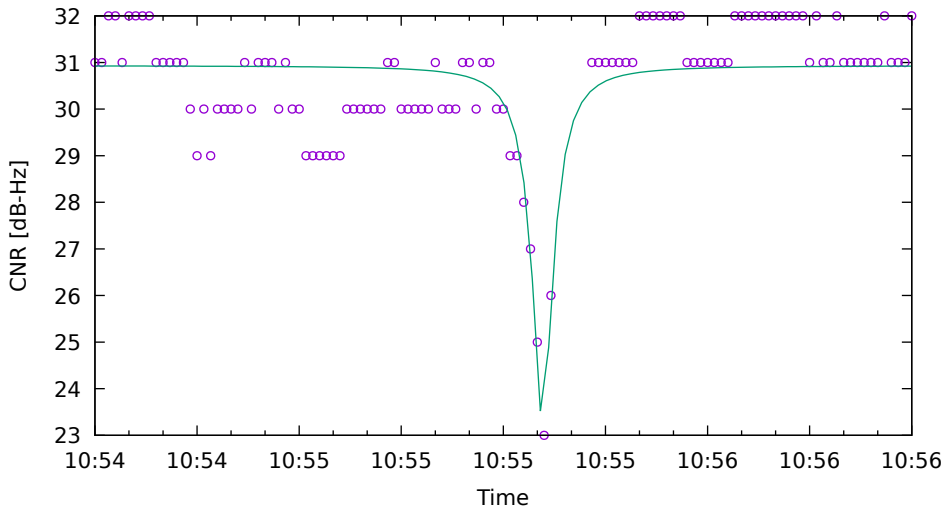
CNR fit for G01 on HuaweiP40 - drive 9 (DOY263)
