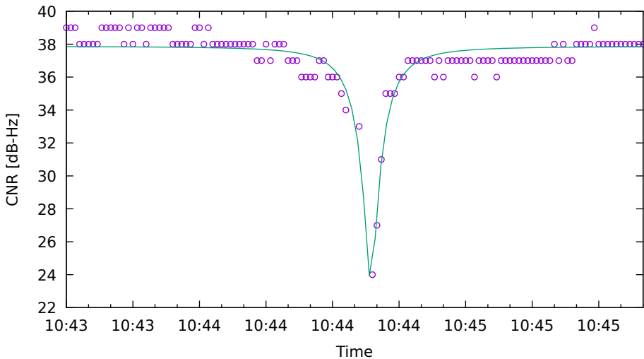
CNR fit for G03 on HuaweiP40 - drive 3 (DOY263)
