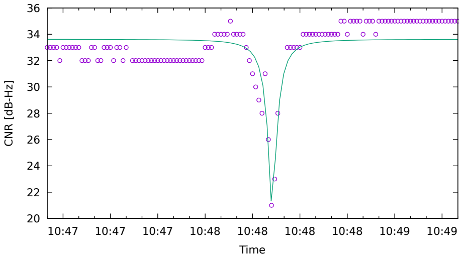
CNR fit for G04 on HuaweiP40 - drive 5 (DOY263)
