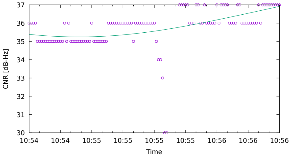
CNR fit for G04 on HuaweiP40 - drive 9 (DOY263)
